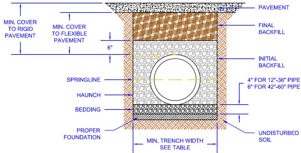
Figure 13 - Typical Trench Installation
