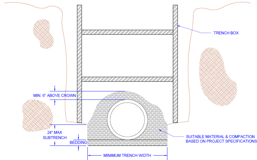
Figure 4 - Typical Sub-Trench Installation
