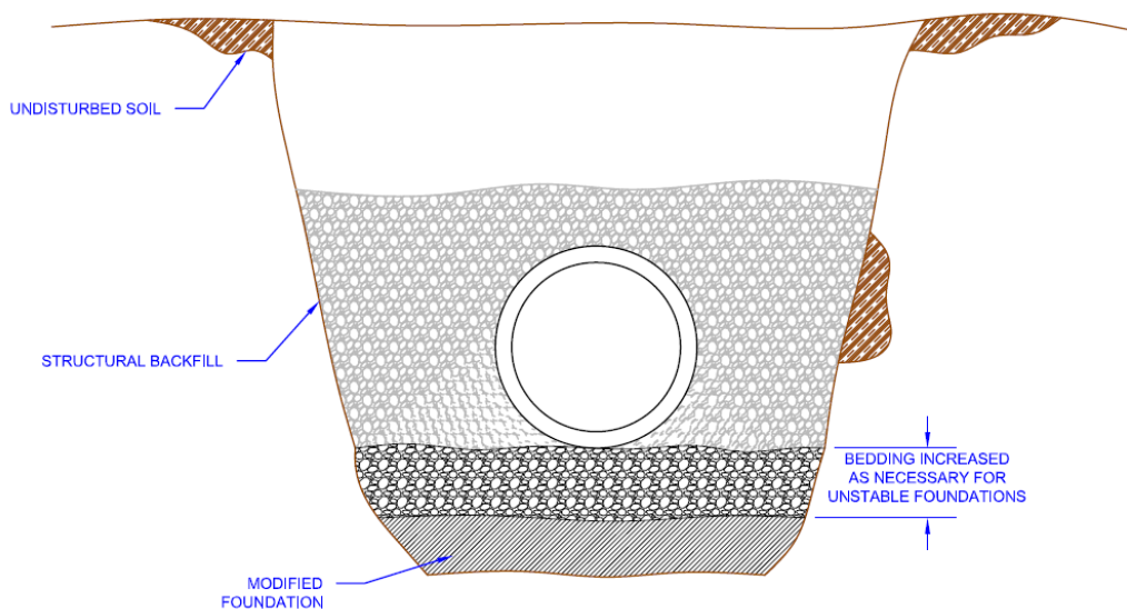
Figure 5 - Modified Foundation
