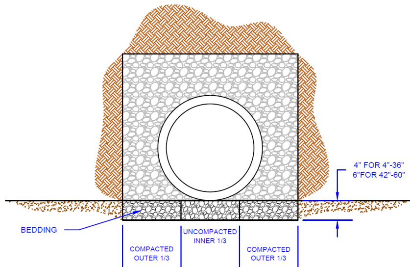
Figure 7 - Bedding Placement
