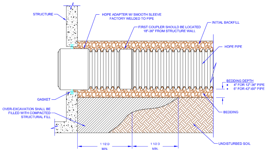
Figure 6 - Typical Structure Connection
