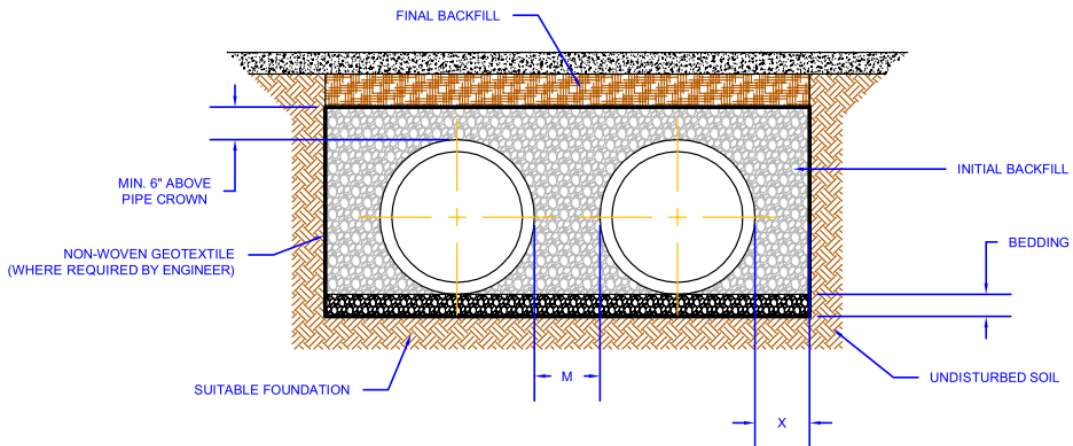
Figure 15 - Typical Parallel Pipe Installation
