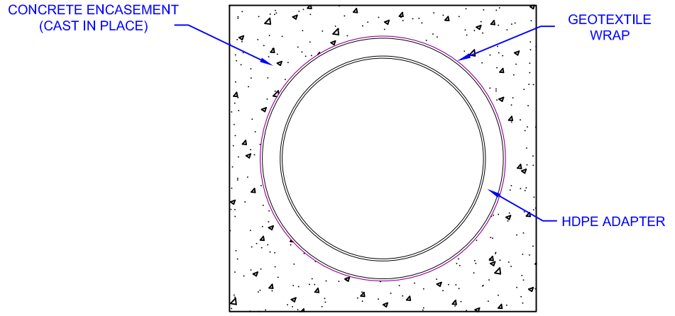
3 CONCRETE ENCASEMENT SECTION DETAIL SCALE: NTS
