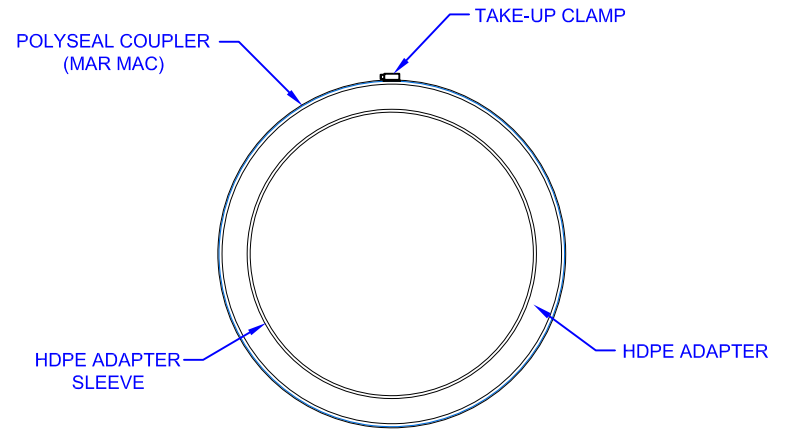
3 POLYSEAL COUPLER SECTION DETAIL 122 SCALE: NTS
