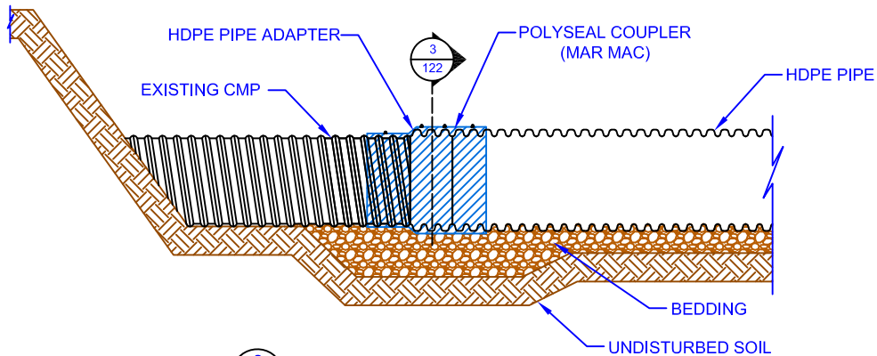
2 HDPE TO CMP ASSEMBLED 122 SCALE: NTS
