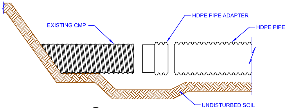
1 HDPE TO CMP PRE ASSEMBLY 122 SCALE: NTS
