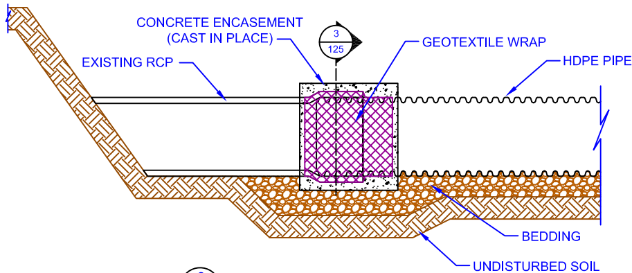
2 HDPE TO RCP ASSEMBLED 125 SCALE: NTS
