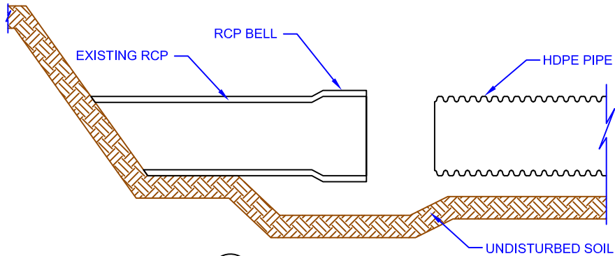
1 HDPE TO RCP PRE ASSEMBLY 125 SCALE: NTS
