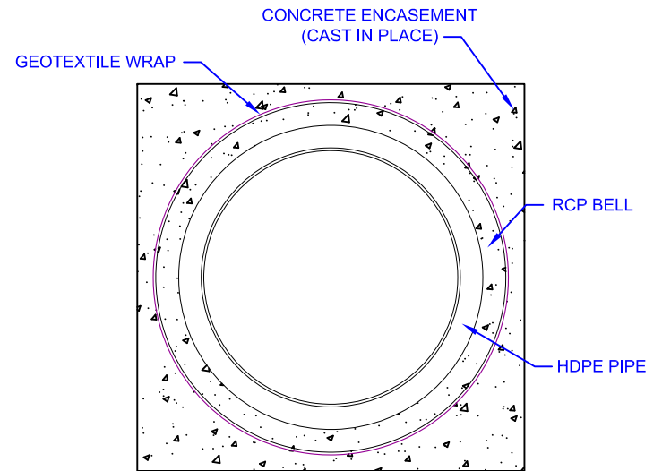
3 CONCRETE ENCASEMENT SECTION DETAIL 125 SCALE: NTS
