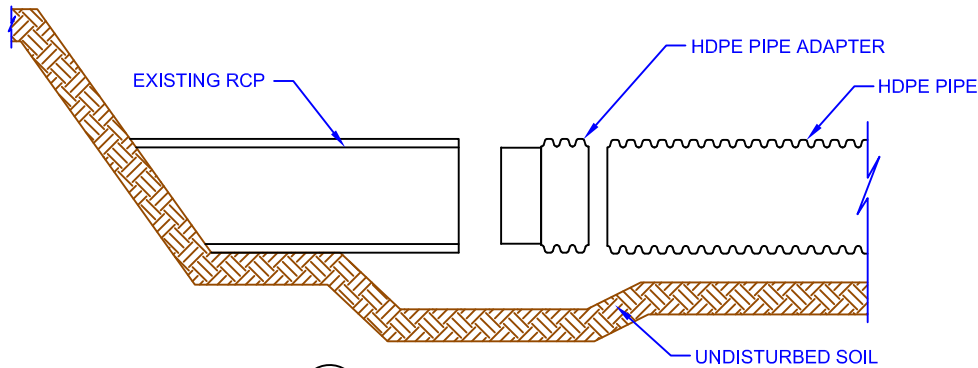
1 124 SCALE: NTS HDPE TO RCP PRE ASSEMBLY
