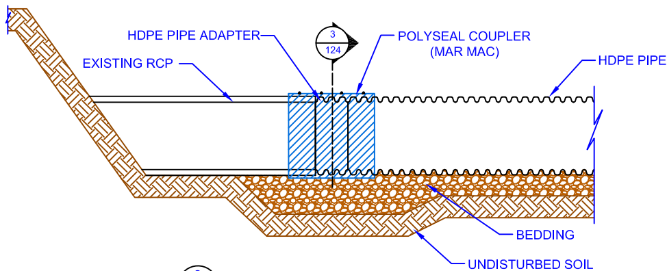
2 124 SCALE: NTS HDPE TO RCP ASSEMBLED
