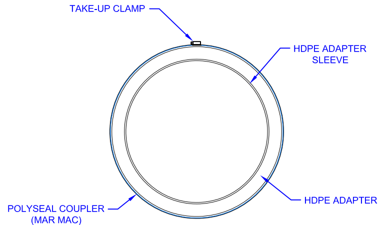
3 124 SCALE: NTS POLYSEAL COUPLER SECTION DETAIL
