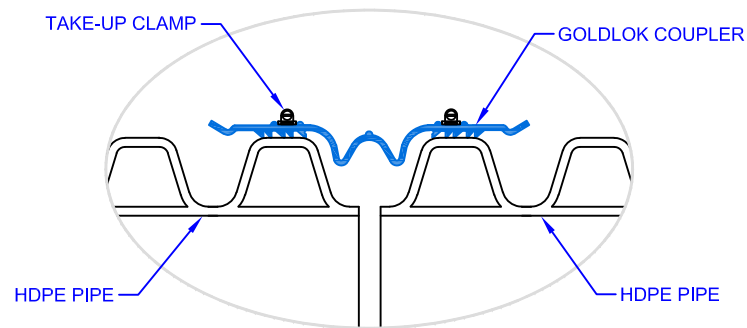
A 128 GOLDLOK SECTION DETAIL SCALE: NTS
