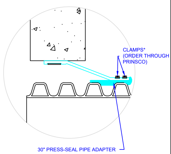
A 120 GASKET DETAIL SCALE: NTS
