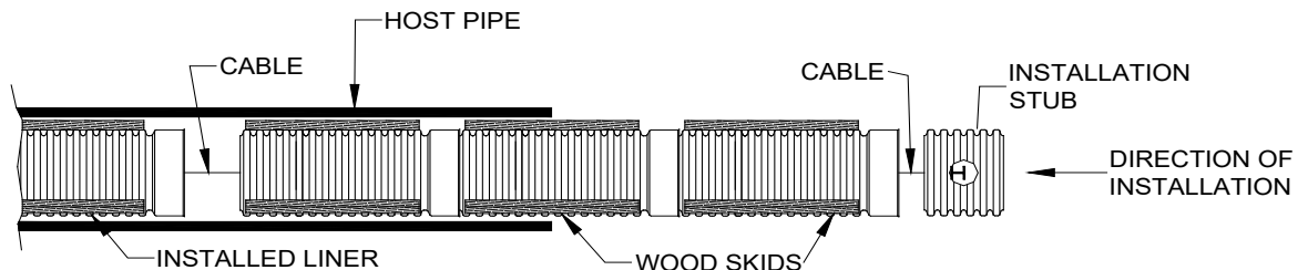
Figure 2: Inserting the Liner into the Host Pipe
