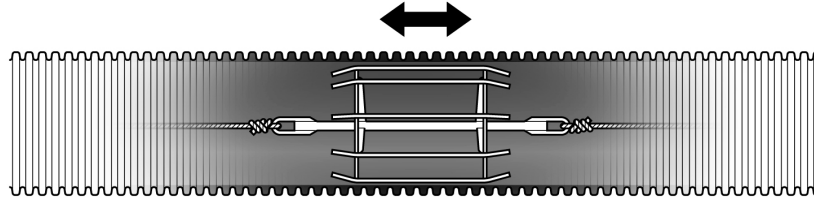
Figure 16: Typical Mandrel
