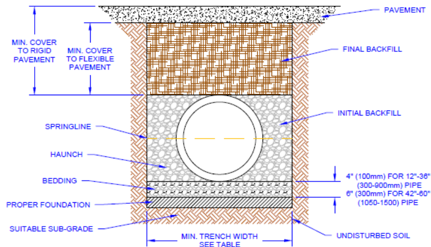
Figure 13: Typical Trench Installation
