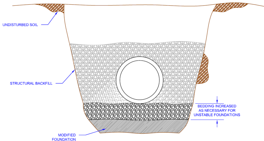
Figure 5: Modified Foundation
