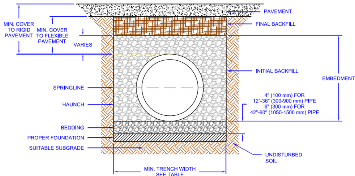
Figure 13: Typical Trench Installation
