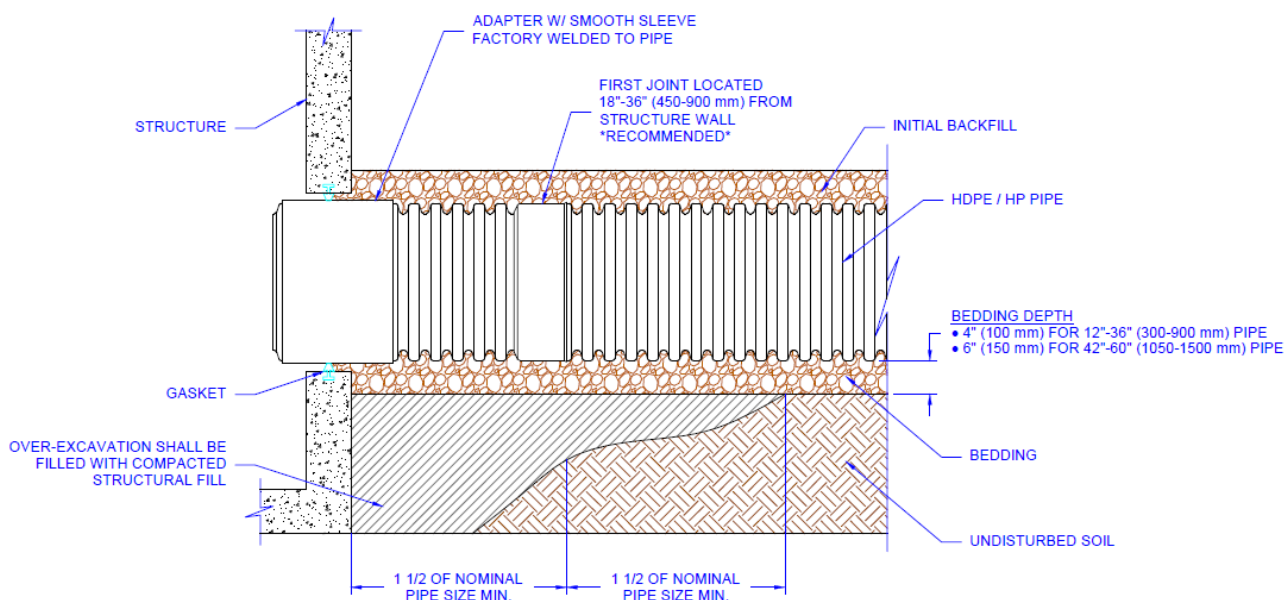
Figure 6: Typical Structure Connection
