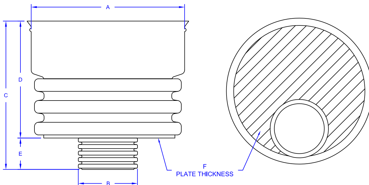
GOLDFLO ECCENTRIC REDUCER 12"-18" - BELLED
