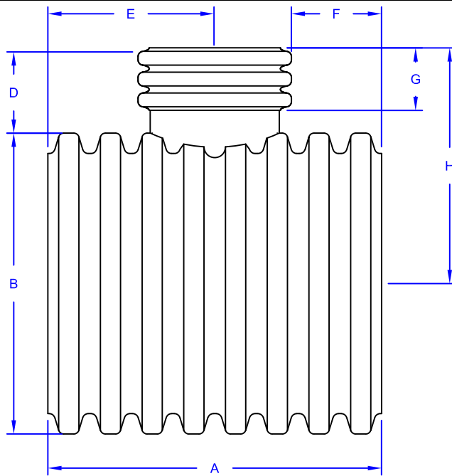
GOLFLO REDUCING TEE 18" - 30" (MW)
