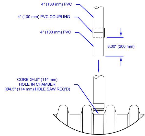
4" PVC COUPLER CONNECTION DETAIL
