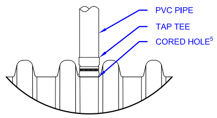
4" (100 mm) TAP TEE CONNECTION DETAIL (SEE NOTE 1)
