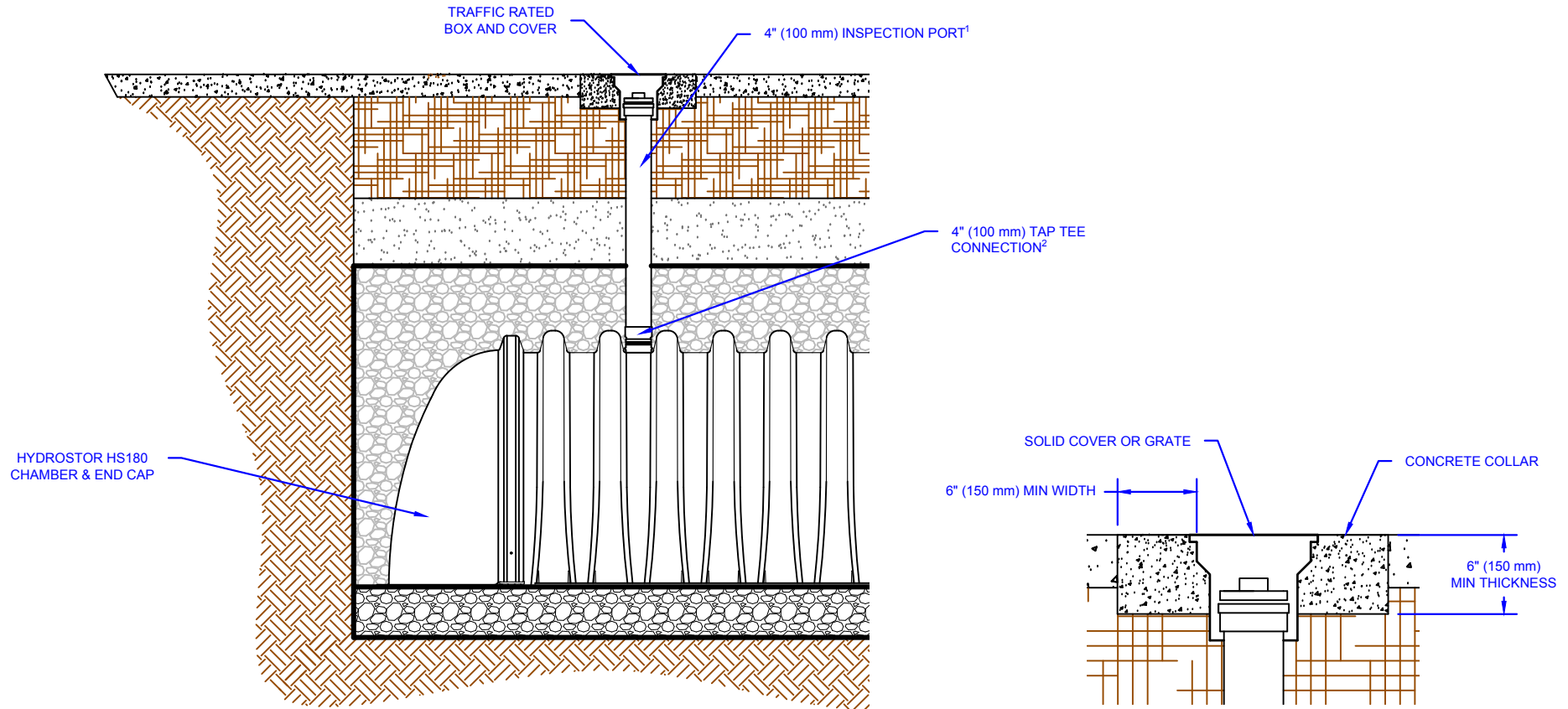
TRAFFIC RATED VALVE BOX DETAIL
