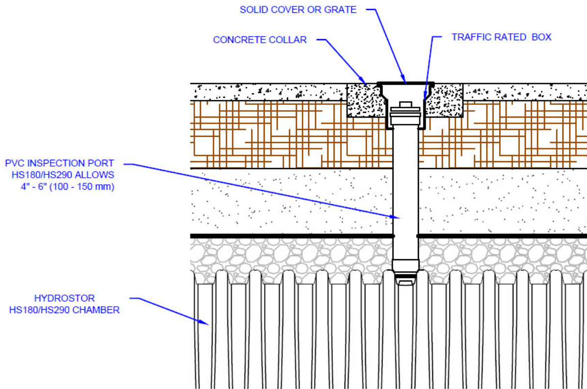
Figure 18 - Inspection Ports
