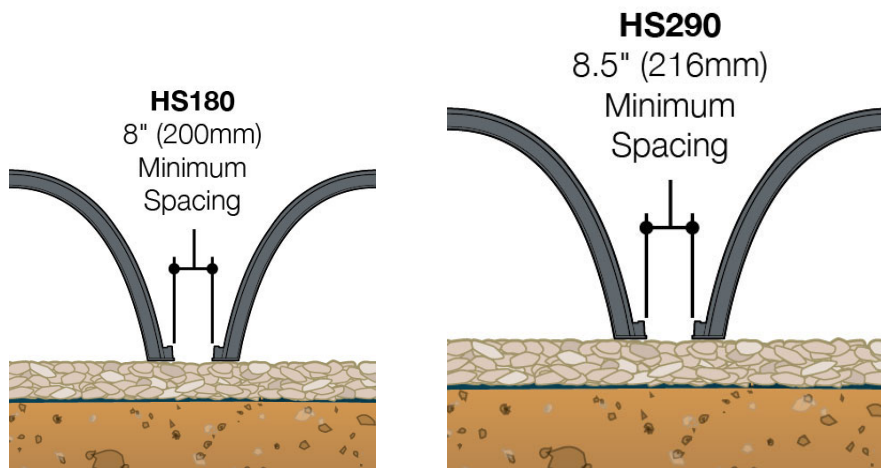
Figure 14 - Minimum Chamber Row Spacing
