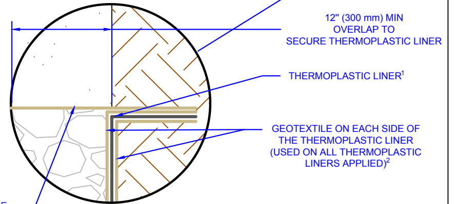
THERMOPLASTIC LINER DETAIL
