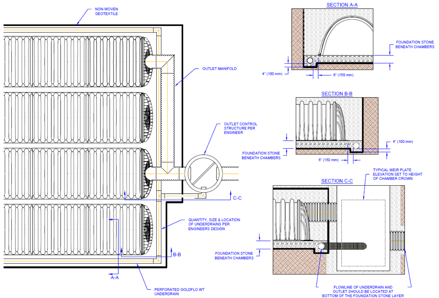
Figure 15 - Optional Underdrain Outlet
