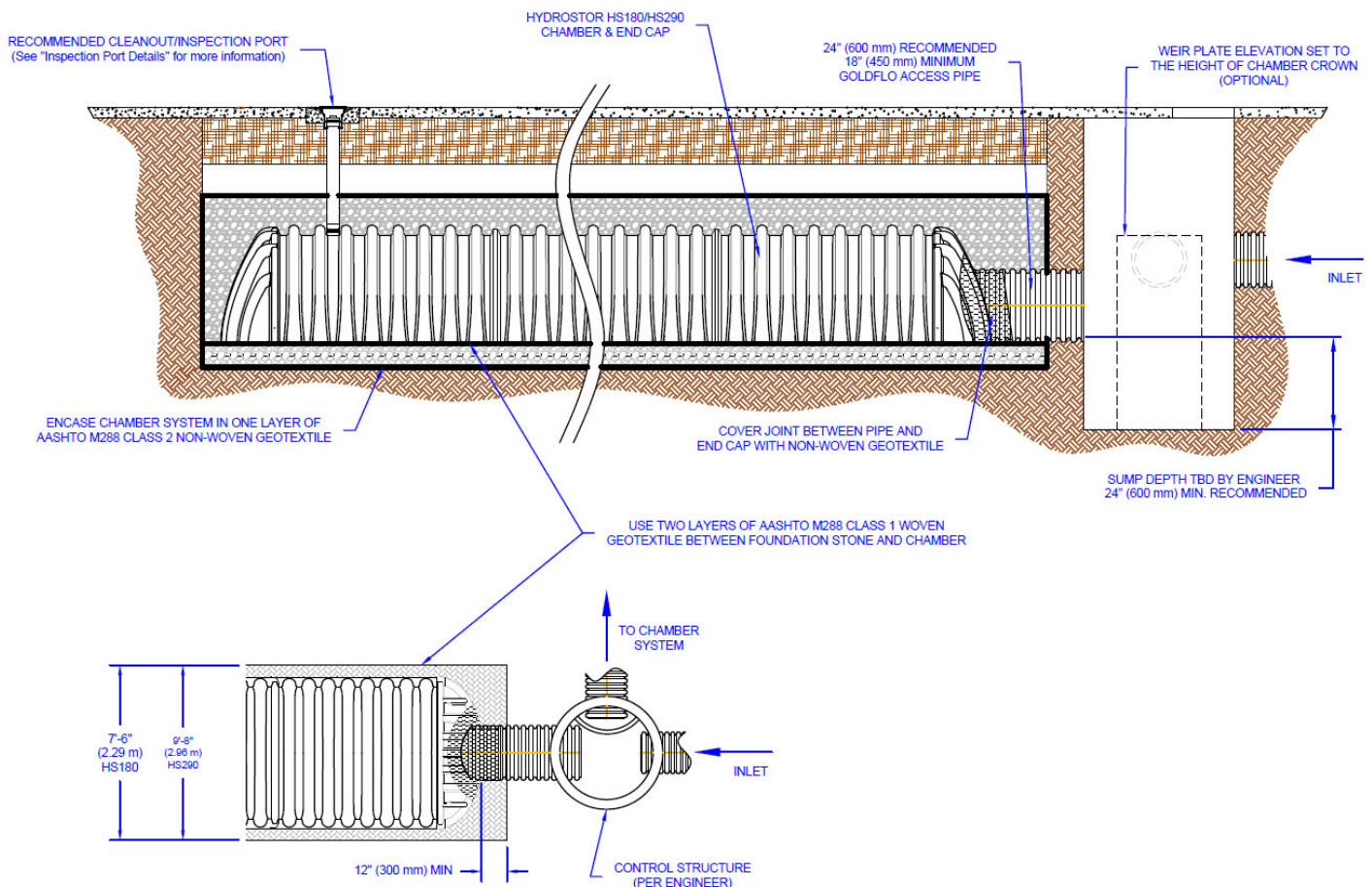
Figure 11 - Sediment Row
