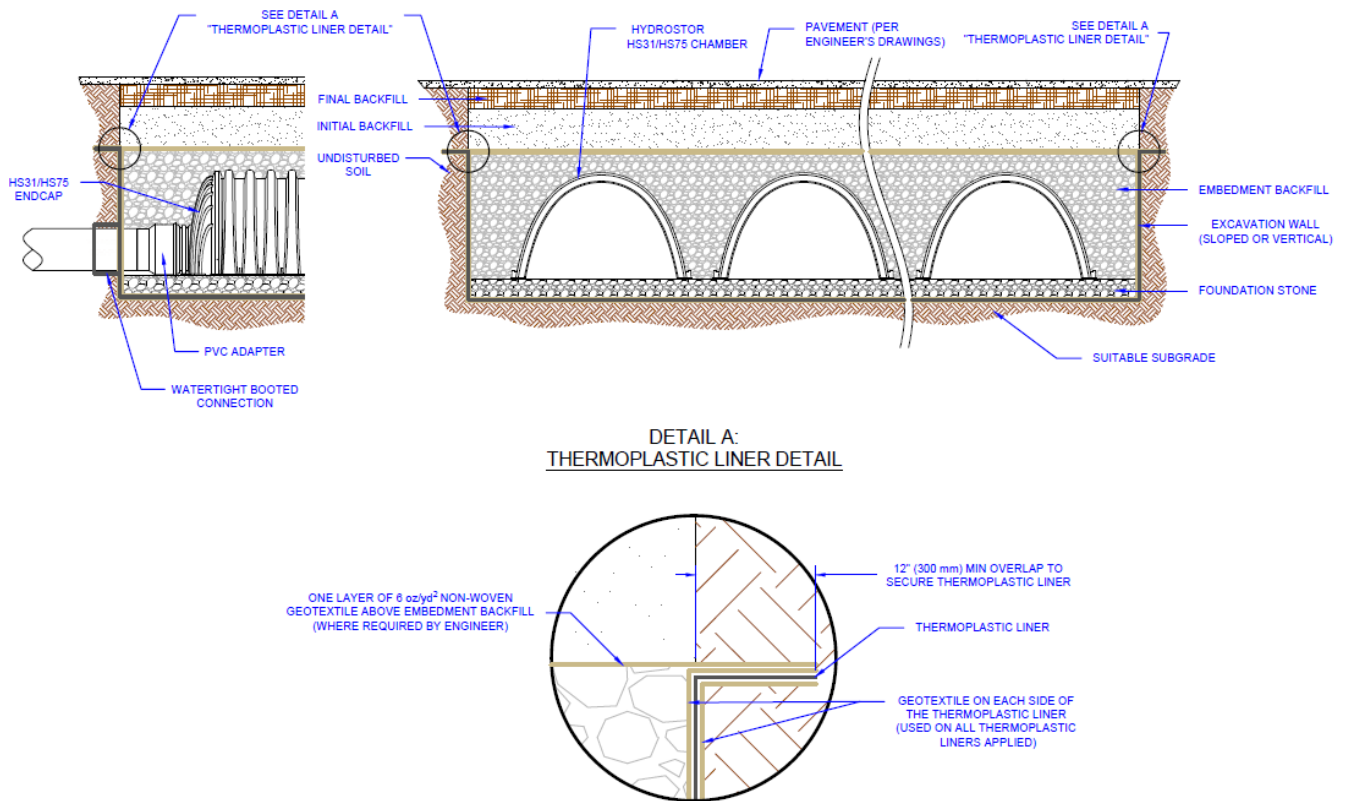
Figure 17 - Impermeable Liner Cross Section
