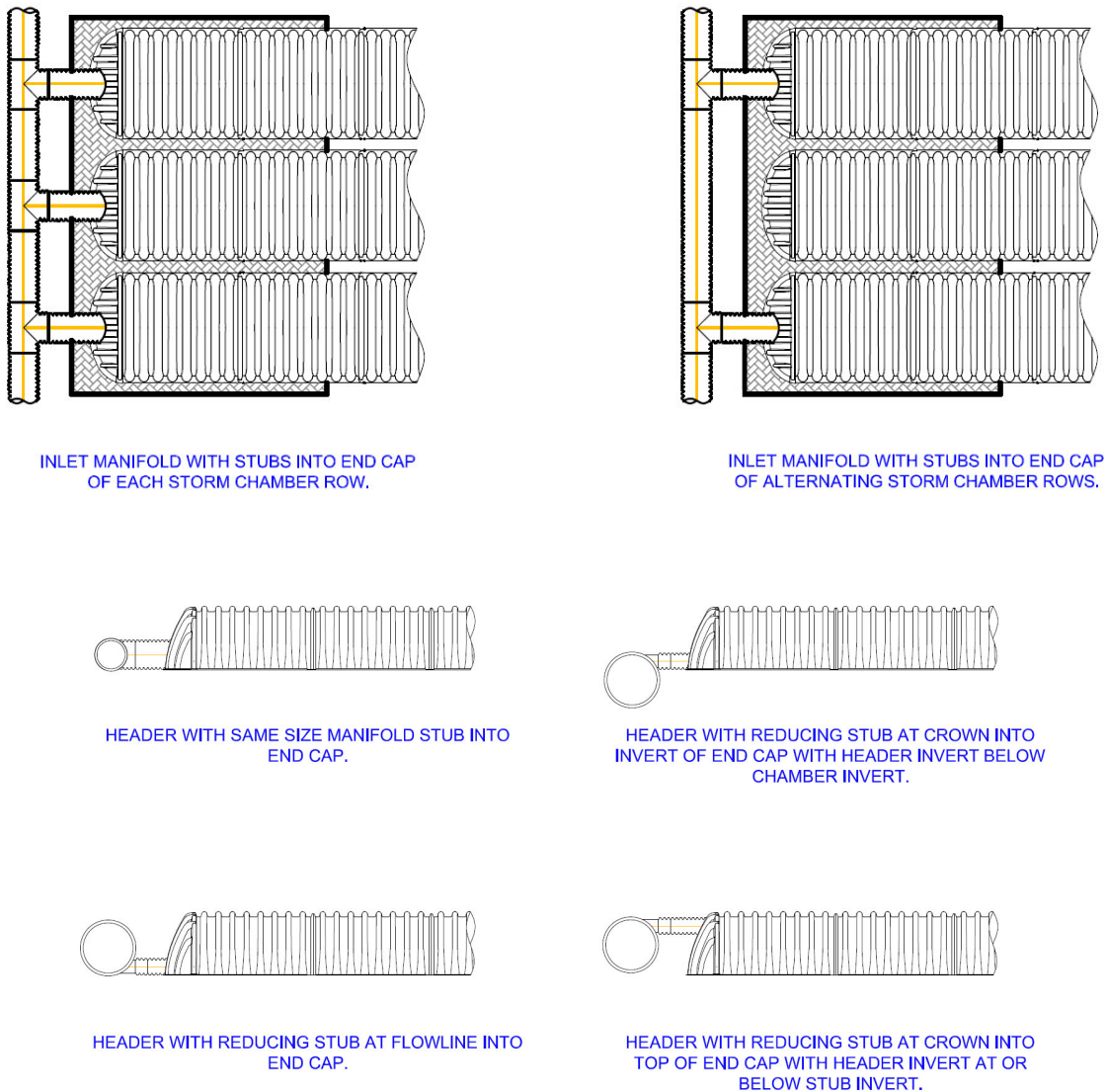
Figure 12 - Inlet Manifold Options
