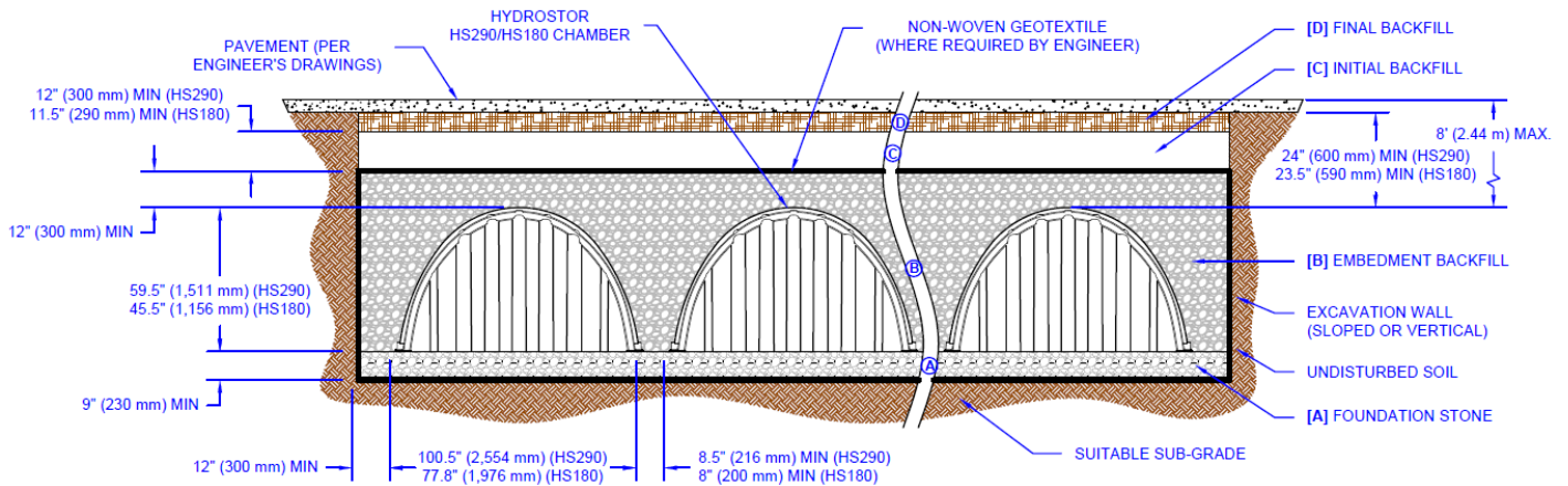
Figure 6 - HydroStor Chamber Cross Section
