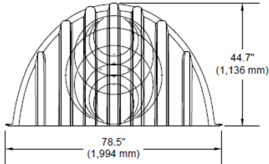
Figure 1 - HydroStor HS180 Chamber & End Caps
