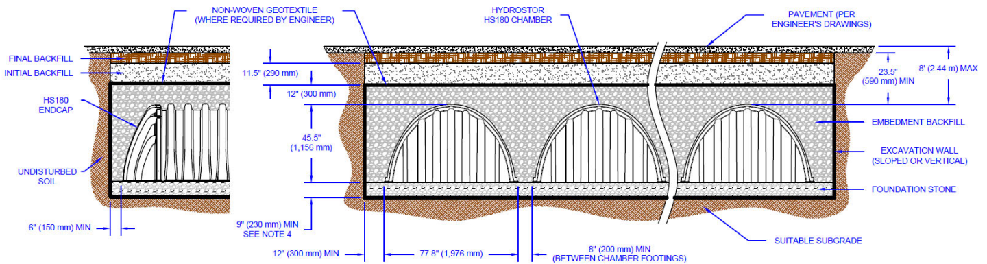
Figure 18 – HS180 Structural Cross Section Detail
