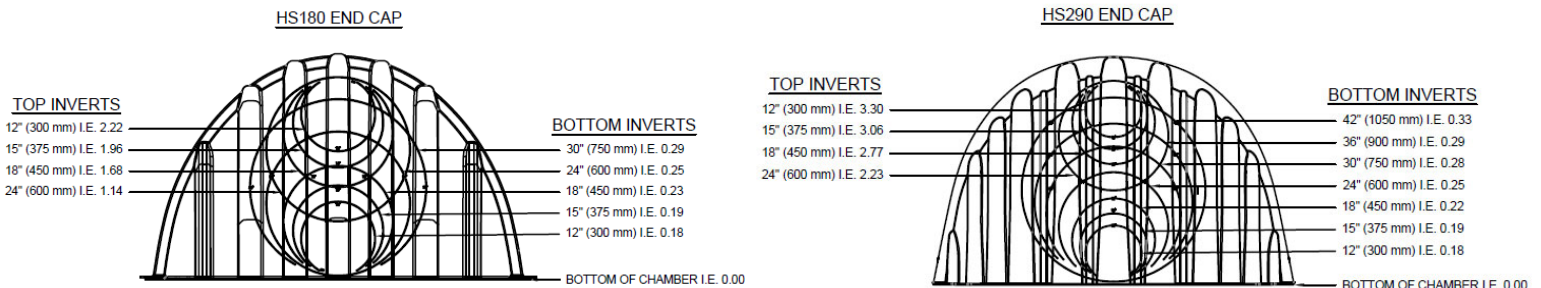
Figure 5 - End Cap Inverts
