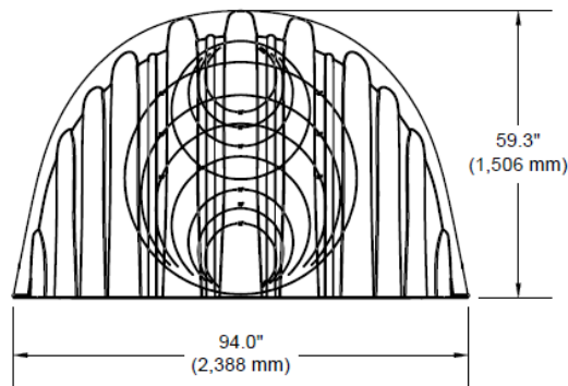
Figure 2 - HydroStor HS290 Chamber & End Caps
