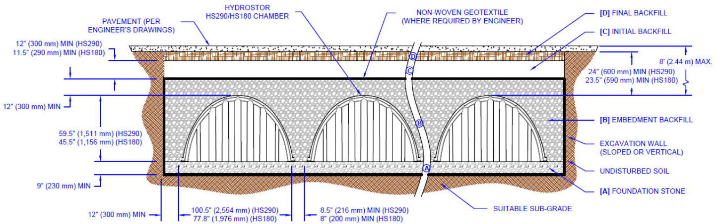
Figure 8 - Chamber Cross Section
