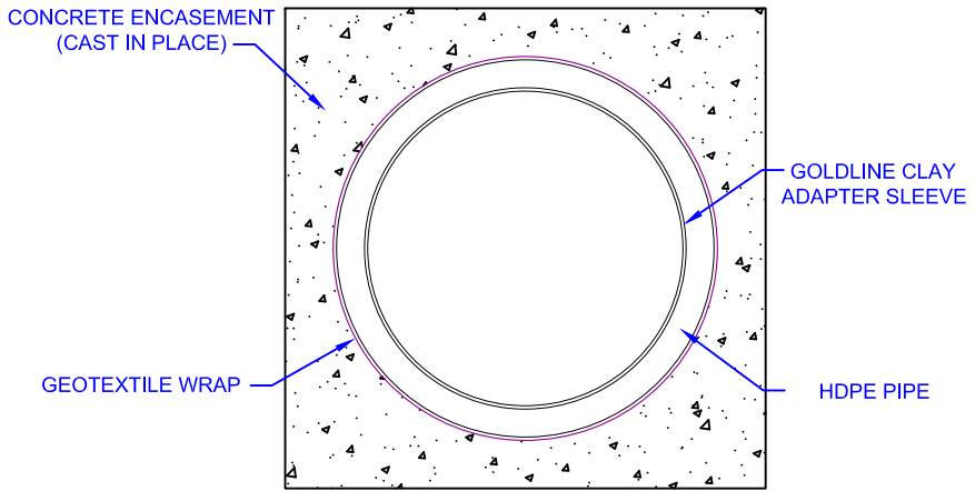
3 CONCRETE ENCASEMENT SECTION DETAIL SCALE: NTS
