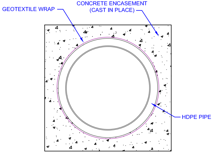
3 CONCRETE ENCASEMENT SECTION DETAIL 140 SCALE: NTS
