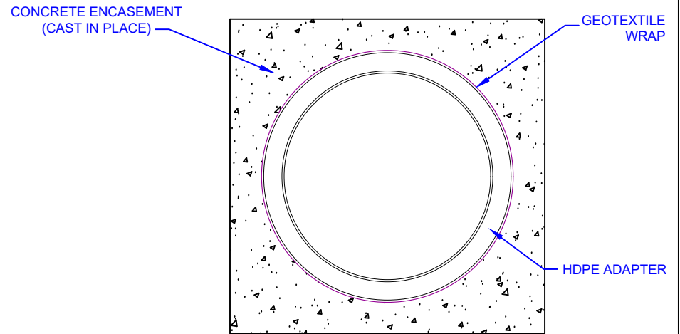
3 CONCRETE ENCASEMENT SECTION DETAIL SCALE: NTS
