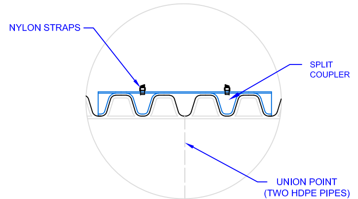
A SPLIT-COUPLER DETAIL 134 SCALE: NTS
