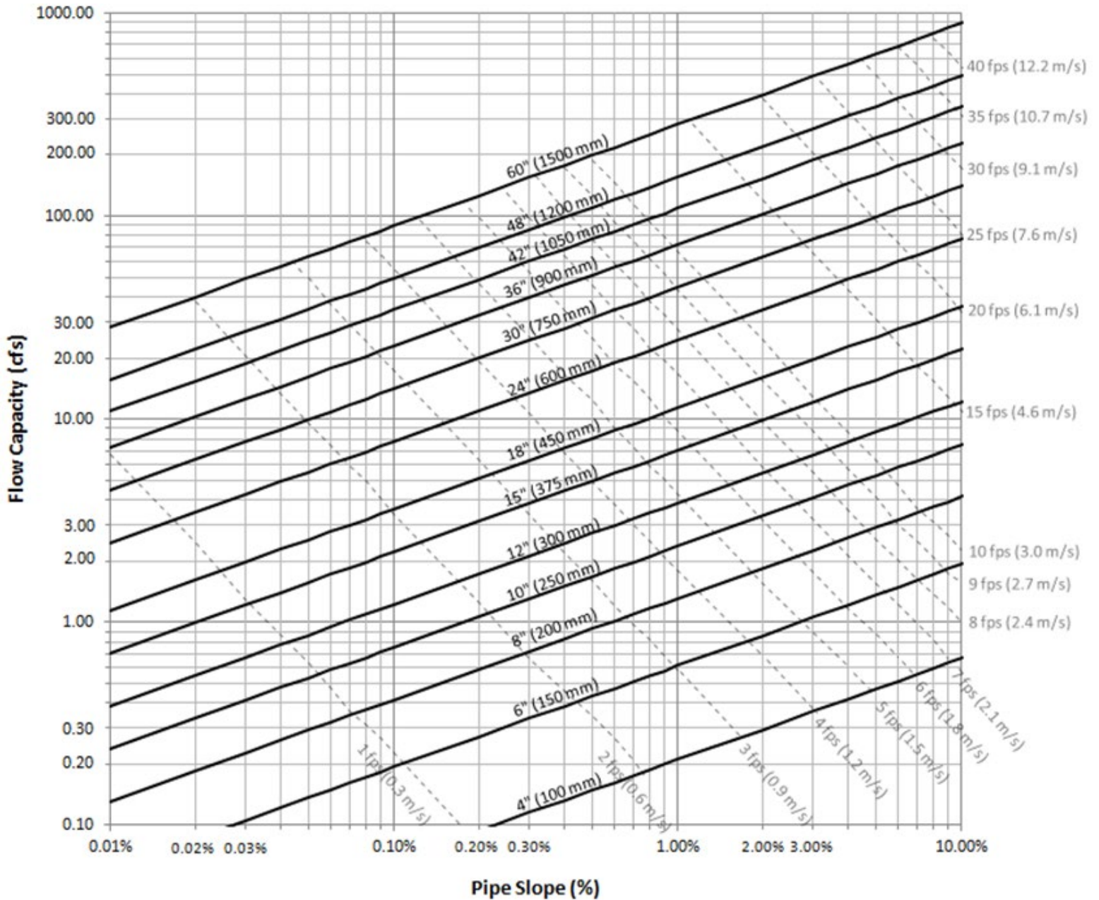
Figure 1: Discharge Curves for Princo Dual Wall Pipe Products (GOLDFLO®, ECOFLO® 100, GOLDPRO Storm™)
