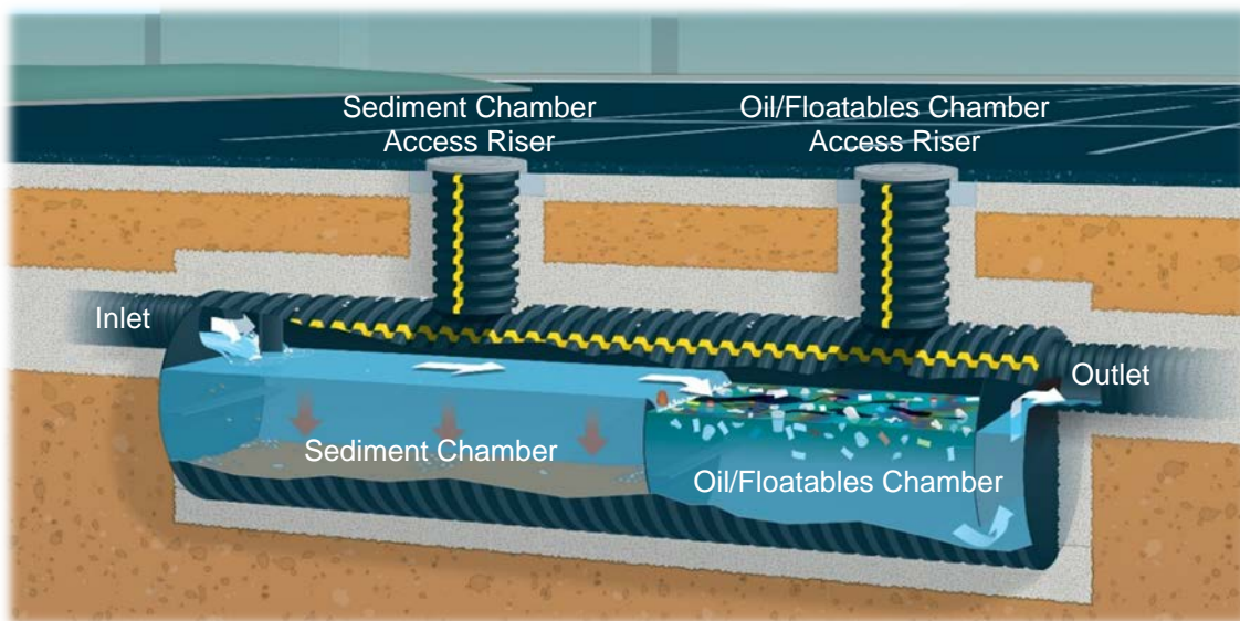
Figure 1: SWQU Components
