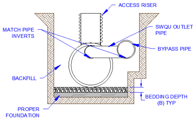
Figure 3: Bedding Placement
