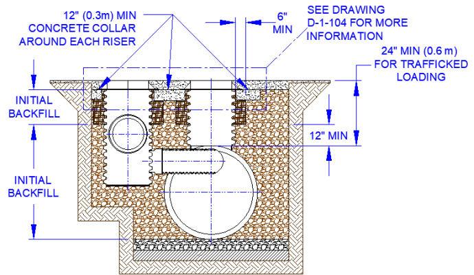
Figure 7: Final Backfill
