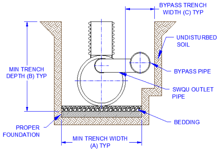
Figure 1: Trench Dimensions
