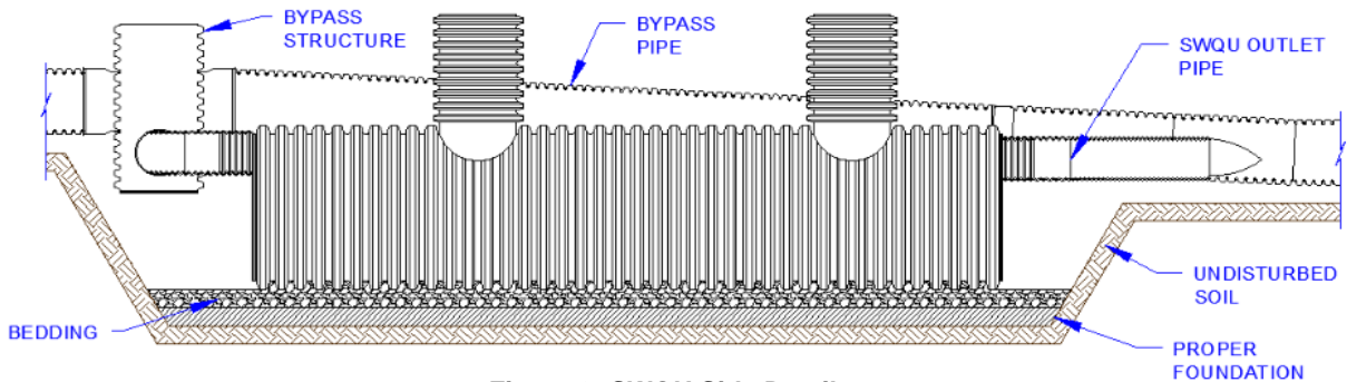
Figure 2: SWQU Side Detail
