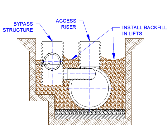
Figure 6: Initial Backfill
