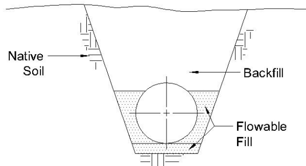
Figure 1: Flowable Fill Backfill
