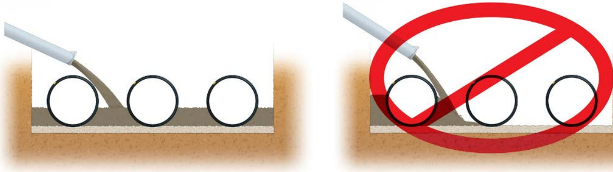
Figure 2: Flowable Fill Placement Recommendation
