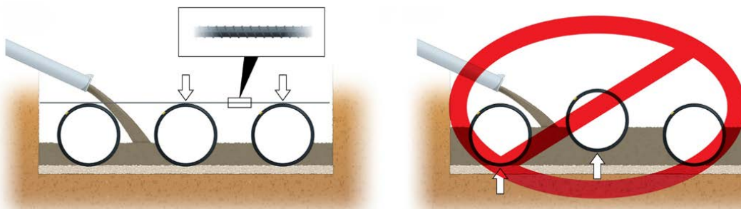
Figure 3: Pipe Anchoring to Prevent Flotation
