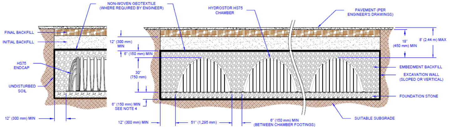
Figure 19 - HS75 Structural Cross Section Detail
