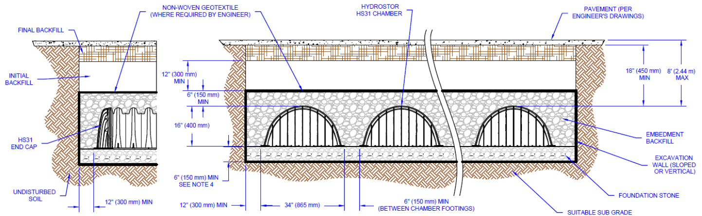
Figure 18 – HS31 Structural Cross Section Detail
