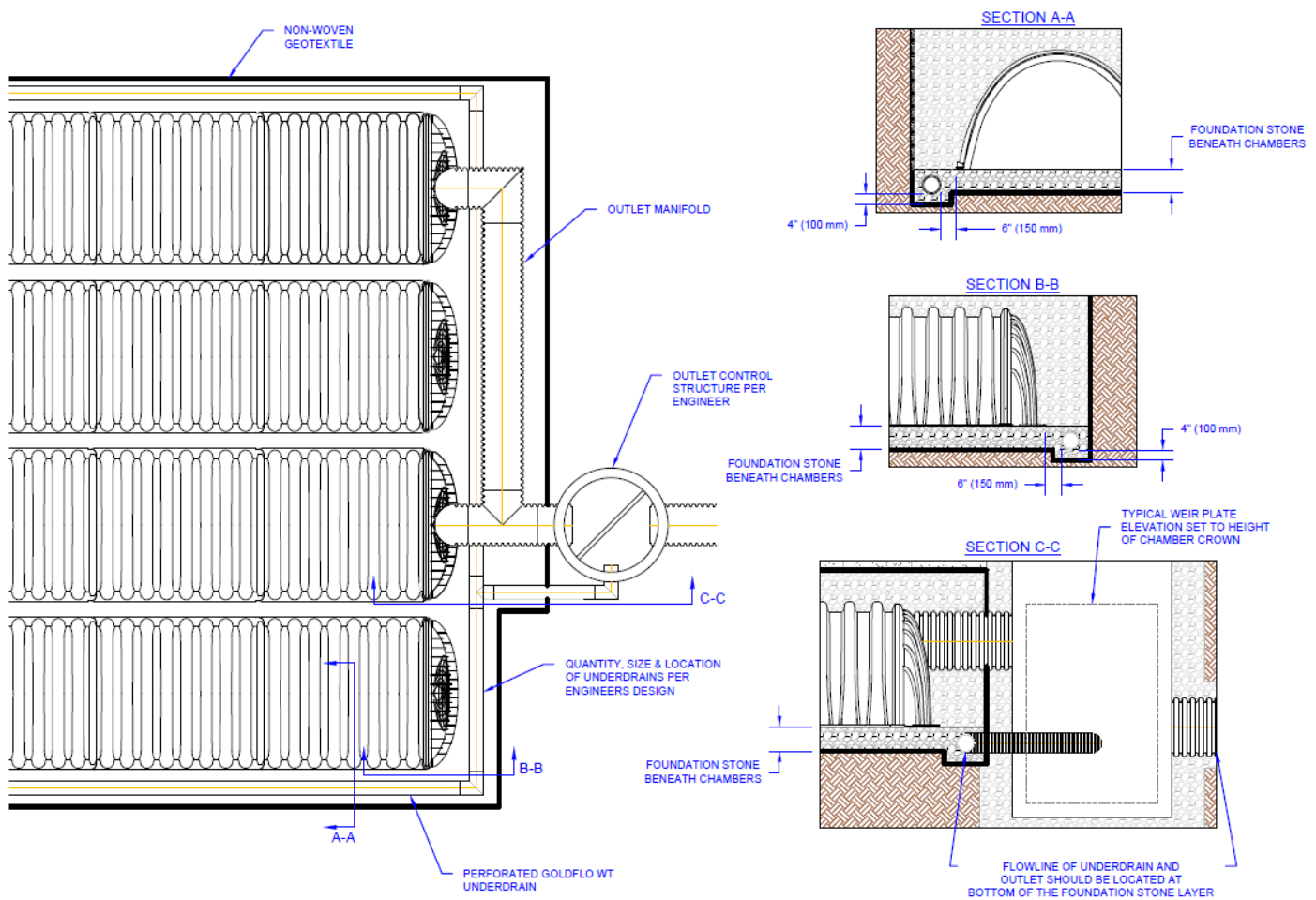
Figure 15 – Optional Underdrain Outlet
