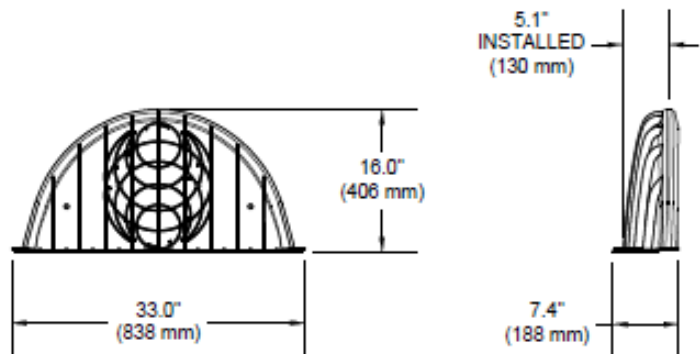
Figure 1- HydroStor HS31 Chamber & End Caps
