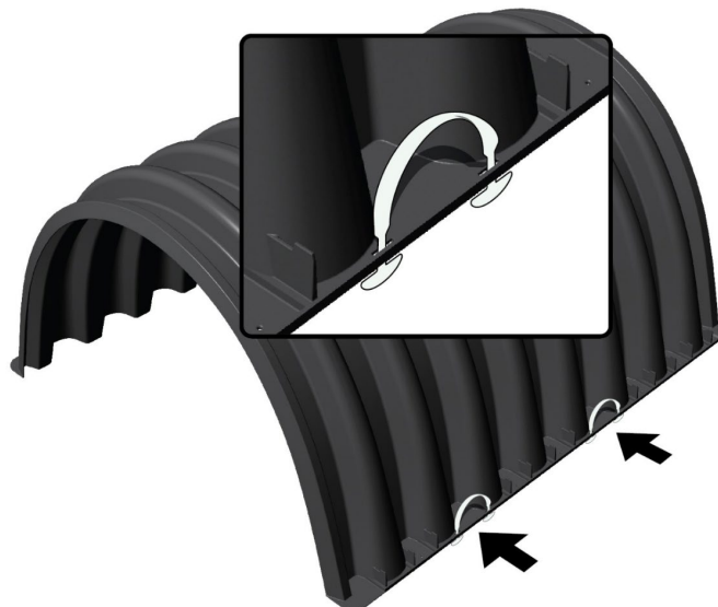
Figure 3 - Chamber Handles
