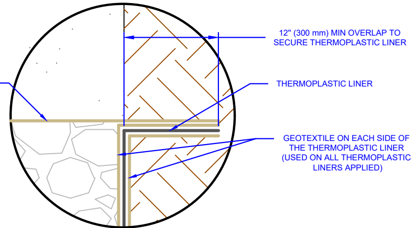
DETAIL A: THERMOPLASTIC LINER DETAIL
