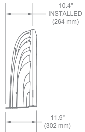
HydroStor® HS75 end cap side view
