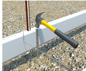
Tap pin to desired elevation
