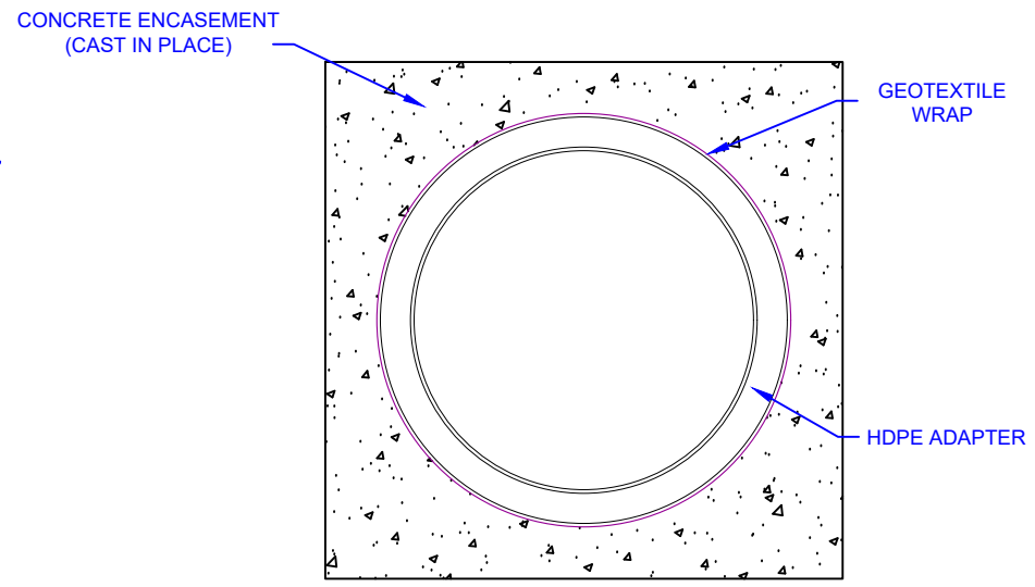
3 CONCRETE ENCASEMENT SECTION DETAIL 121 SCALE: NTS
