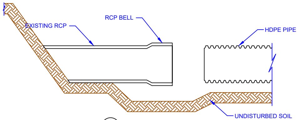
1 HDPE TO RCP PRE ASSEMBLY SCALE: NTS
