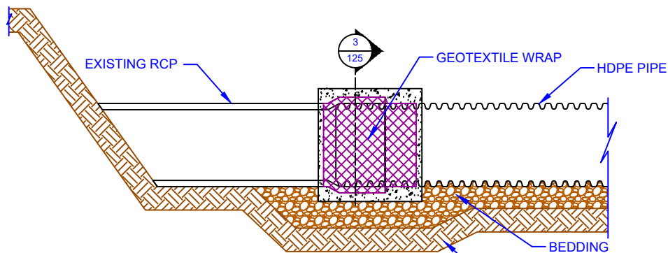
2 HDPE TO RCP ASSEMBLED SCALE: NTS
