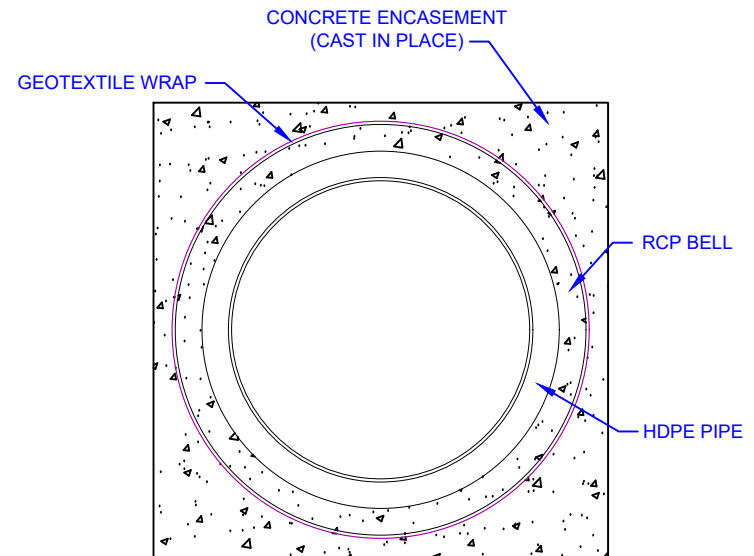
3 CONCRETE ENCASEMENT SECTION DETAIL SCALE: NTS
