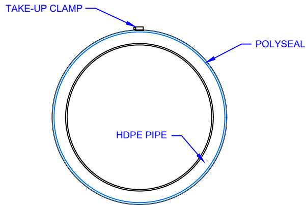
A (MAR MAC) POLYSEAL DETAIL 127 SCALE: NTS
