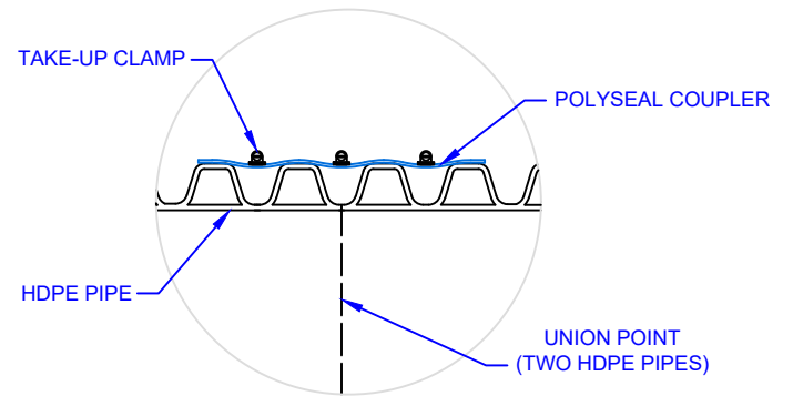
B POLYSEAL SECTION DETAIL 127 SCALE: NTS
