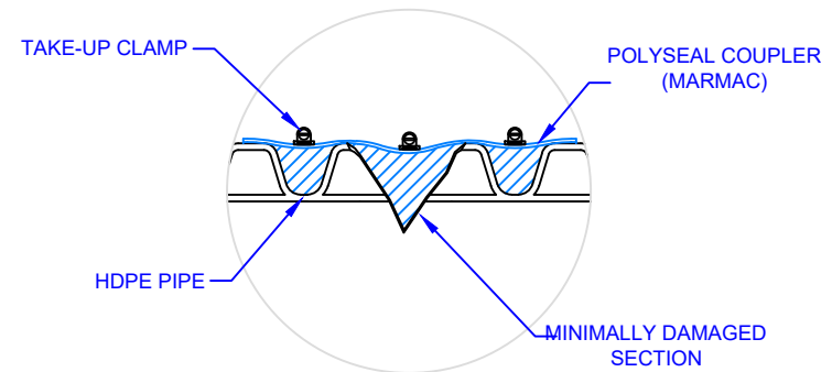
B POLYSEAL SECTION DETAIL 136 SCALE: NTS
