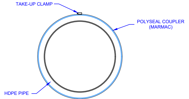
A POLYSEAL DETAIL 136 SCALE: NTS
