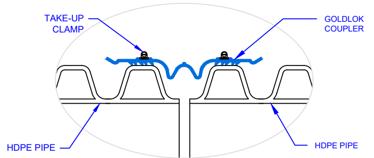
A 133 GOLDLOK SECTION DETAIL SCALE: NTS
