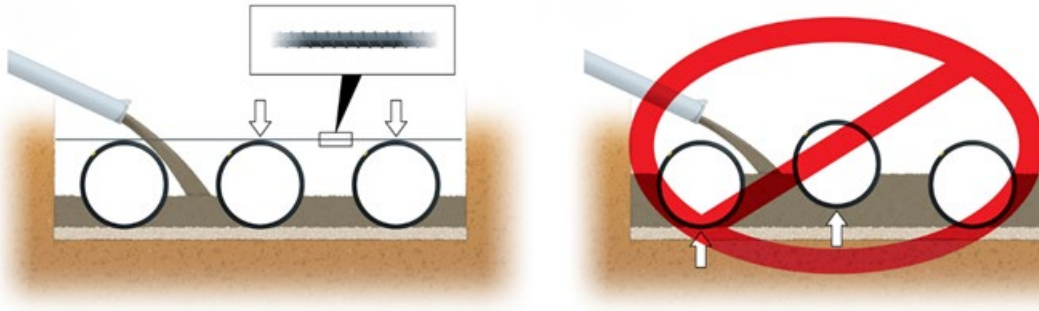
Figure 3: Pipe Restraint to Prevent Flotation
