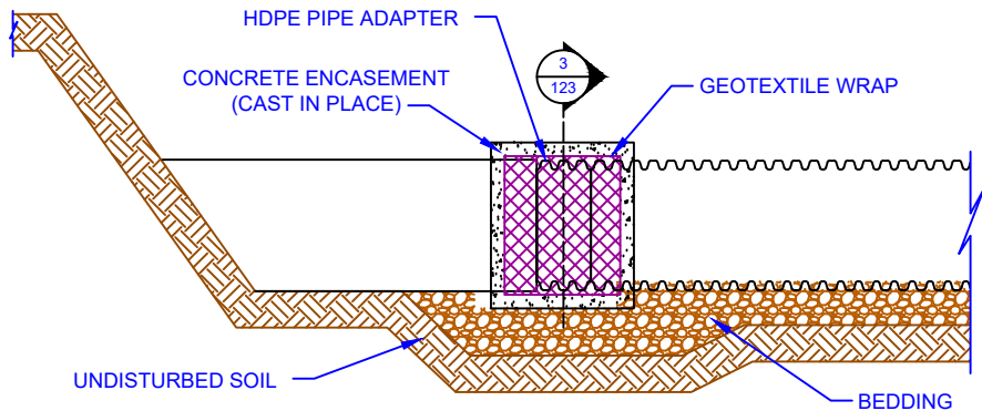
2 HDPE TO RCP ASSEMBLED SCALE: NTS
