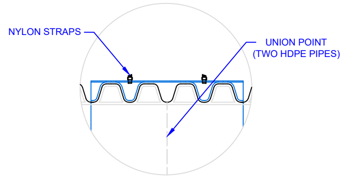
B 126 SCALE: NTS SPLIT-COUPLER DETAIL
