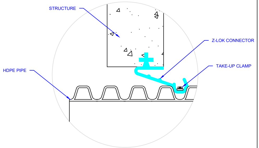
A GASKET DETAIL 119 SCALE: NTS
