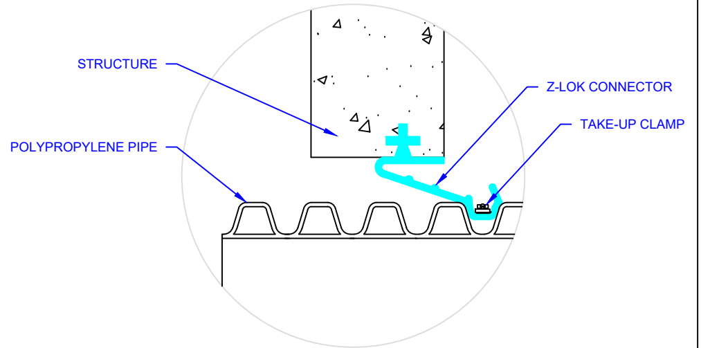
A 119 GASKET DETAIL SCALE: NTS
