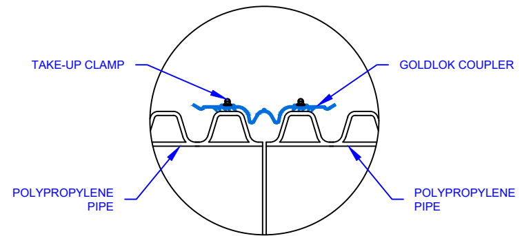
B 128 GOLDLOK SECTION DETAIL SCALE: NTS
