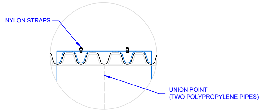
B 126 SCALE: NTS SPLIT-COUPLER DETAIL
