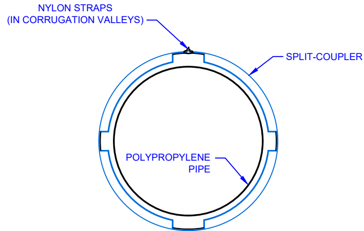
A 126 SCALE: NTS SPLIT-COUPLER DETAIL
