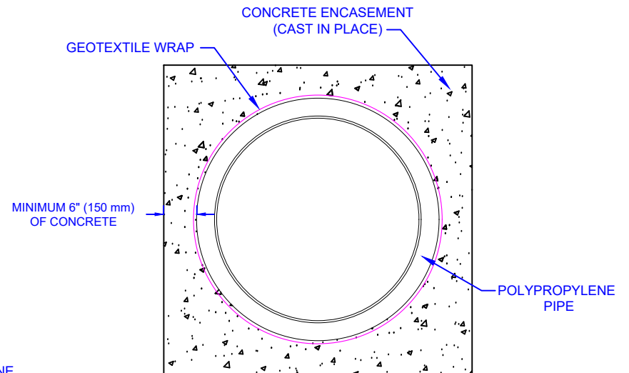
A 135 CONCRETE ENCASEMENT SECTION DETAIL SCALE: NTS
