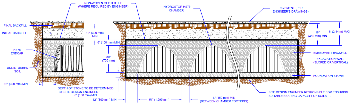
Figure 18 - HS75 Structural Cross Section Detail
