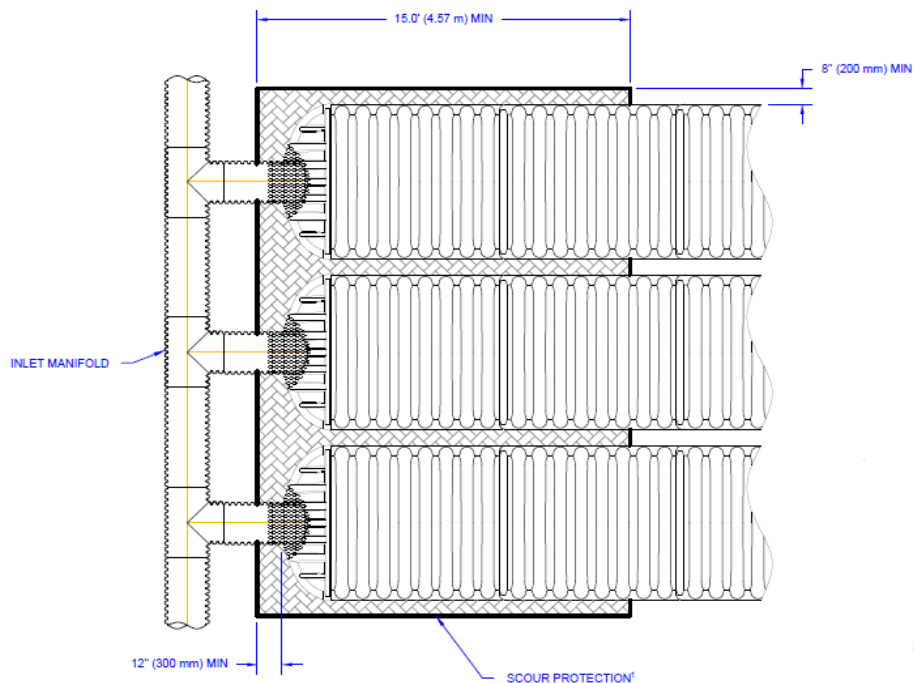
Figure 13 - Inlet Scour Protection
