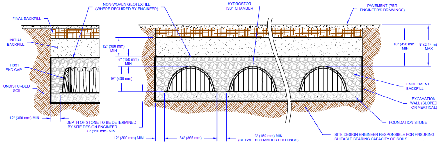
Figure 17 – HS31 Structural Cross Section Detail
