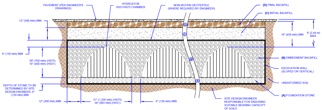
Figure 6 - HydroStor Chamber Cross Section
