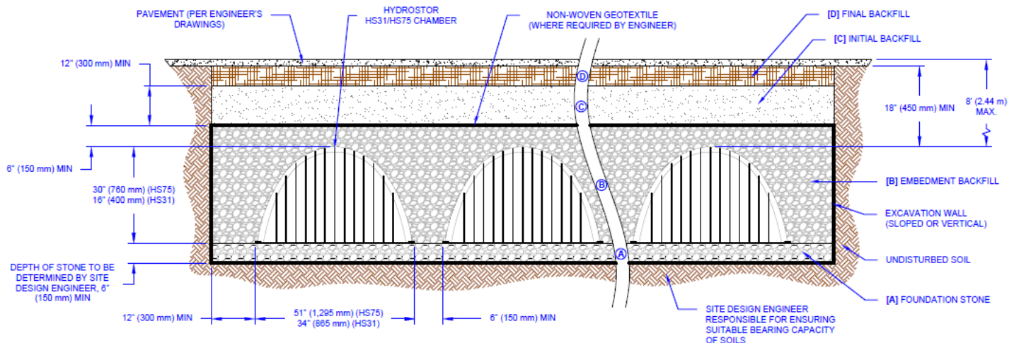
Figure 19 - Chamber Cross Section
