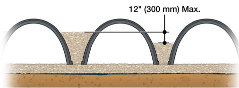
Figure 21 - Embedment Stone Placement
