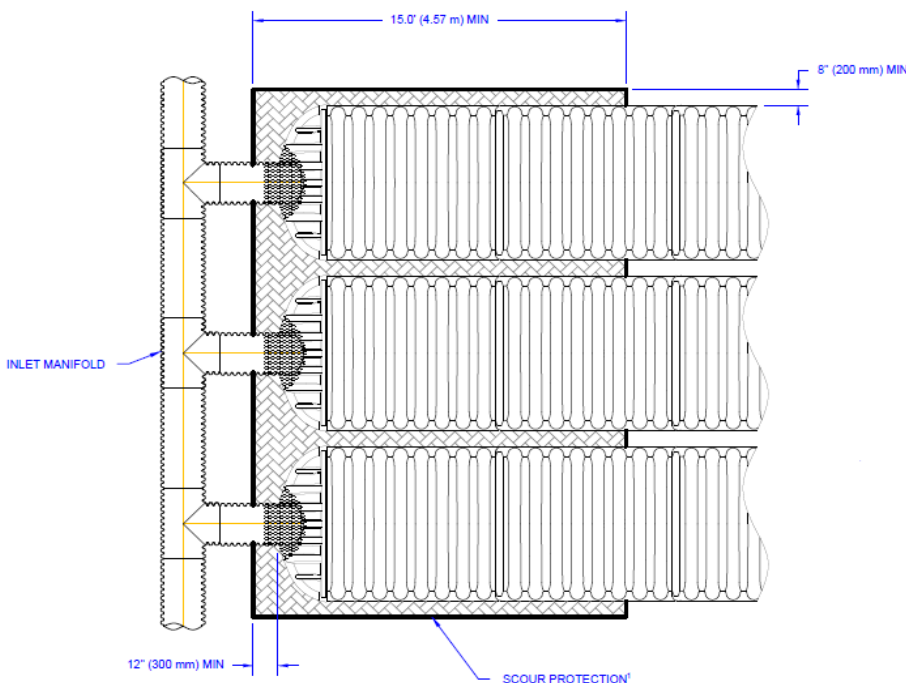
Figure 10 - Inlet Scour Protection
