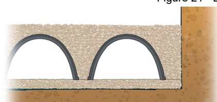
Figure 22 - Perimeter Backfill Placement
