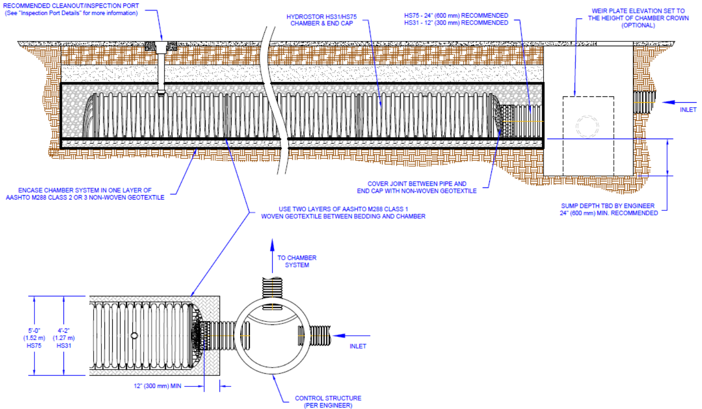
Figure 17 - Sediment Row
