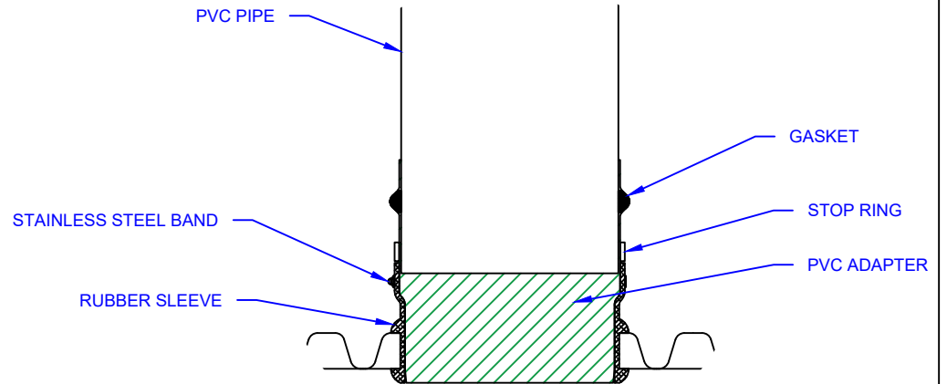
A FULL CONNECTION DETAIL 161 SCALE: NTS
