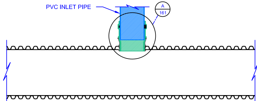
2 PVC ADAPTER INSTALLED 161 SCALE: NTS
