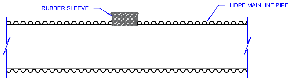
1 RUBBER SLEEVE INSTALLED 161 SCALE: NTS
