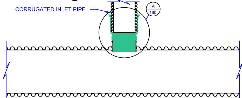
2 PVC ADAPTER INSTALLED SCALE: NTS
