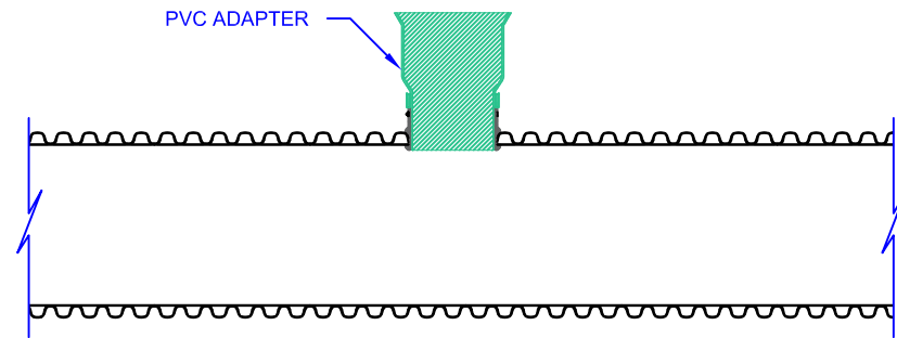
2 PVC ADAPTER INSTALLED SCALE: NTS
