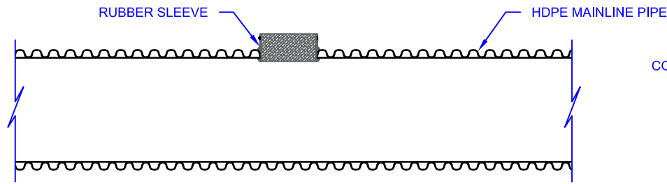
1 RUBBER SLEEVE INSTALLED SCALE: NTS
