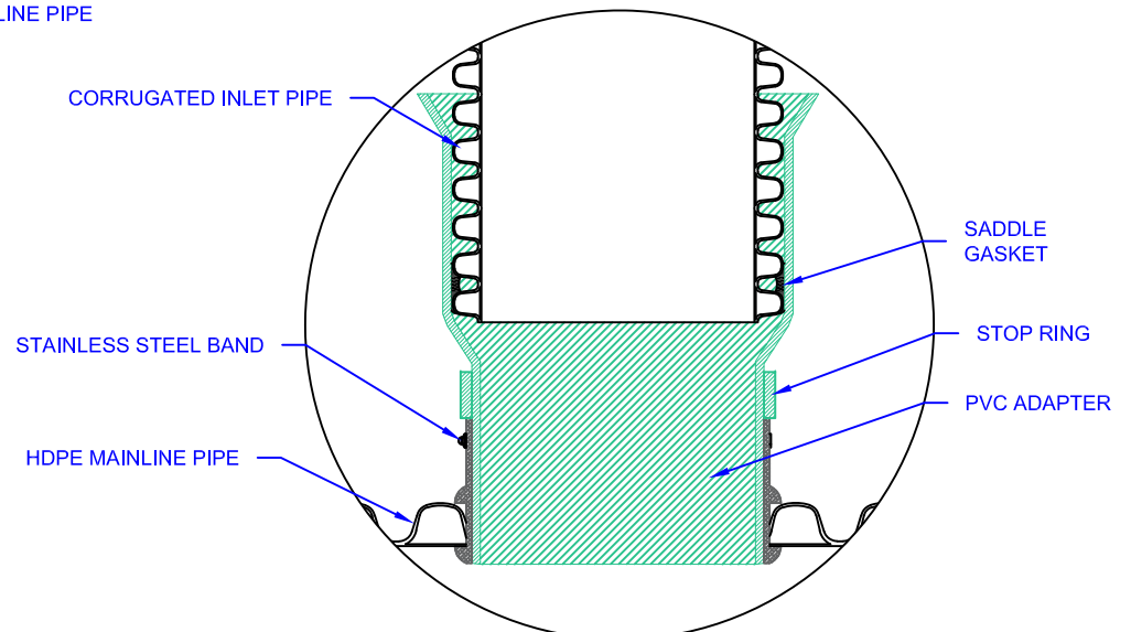
A FULL CONNECTION DETAIL SCALE: NTS
