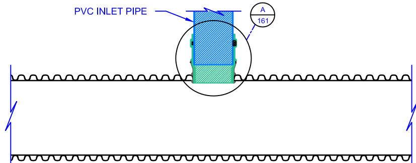
2 PVC ADAPTER INSTALLED SCALE: NTS
