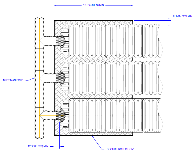
Figure 10 - Inlet Scour Protection
