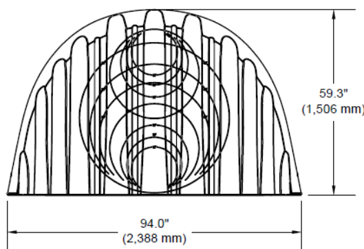
Figure 2 - HydroStor HS290 Chamber & End Caps
