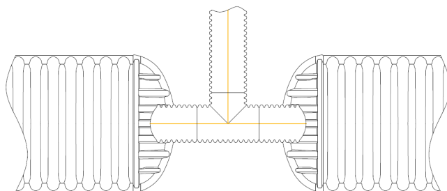
Figure 12– Perpendicular Chamber Connection
