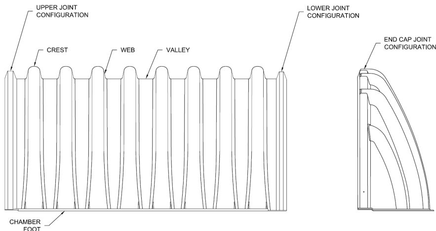
Figure 3 - Chamber and End Cap Components
