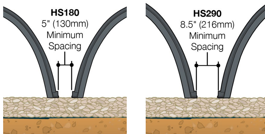
Figure 7- Minimum Chamber Row Spacing
