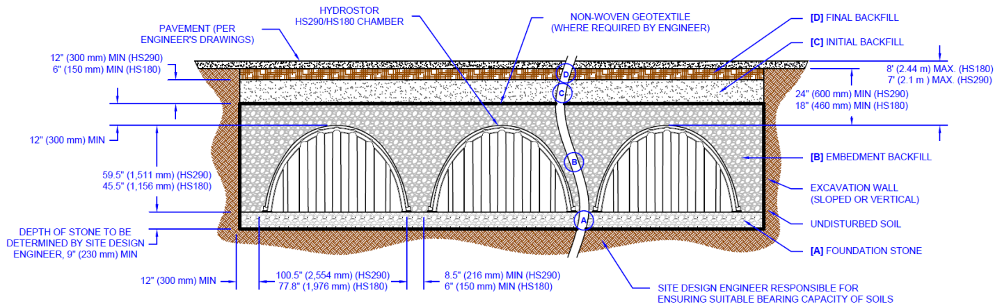
Figure 6- HS180 & HS290 Combined Chamber Cross Section
