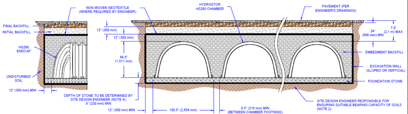
Figure 18– HS290 Structural Cross Section Detail
