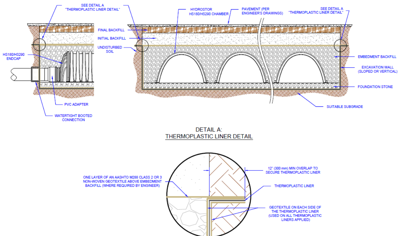
Figure 16- Impermeable Liner Cross Section
