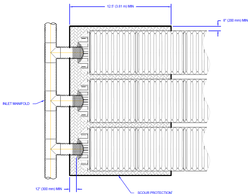
Figure 13. Inlet Scour Protection
