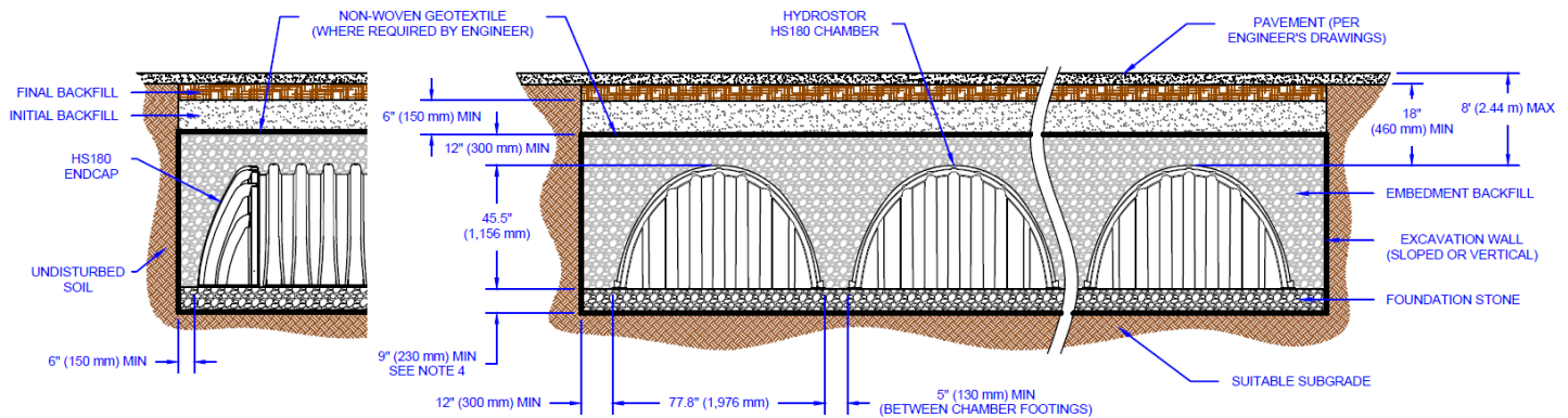
Figure 17– HS180 Structural Cross Section Detail
