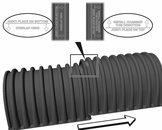
Figure 4 - Chamber Joint Assembly
